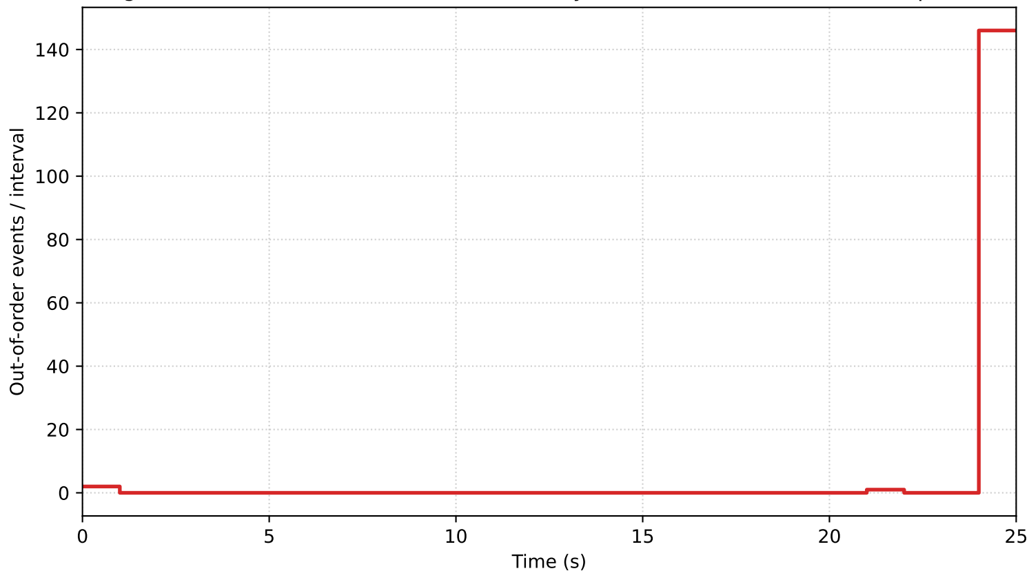
Figure G1 — Out-of-order vs time (LEO-only) — 25 s sim, 1000 ms state updates
